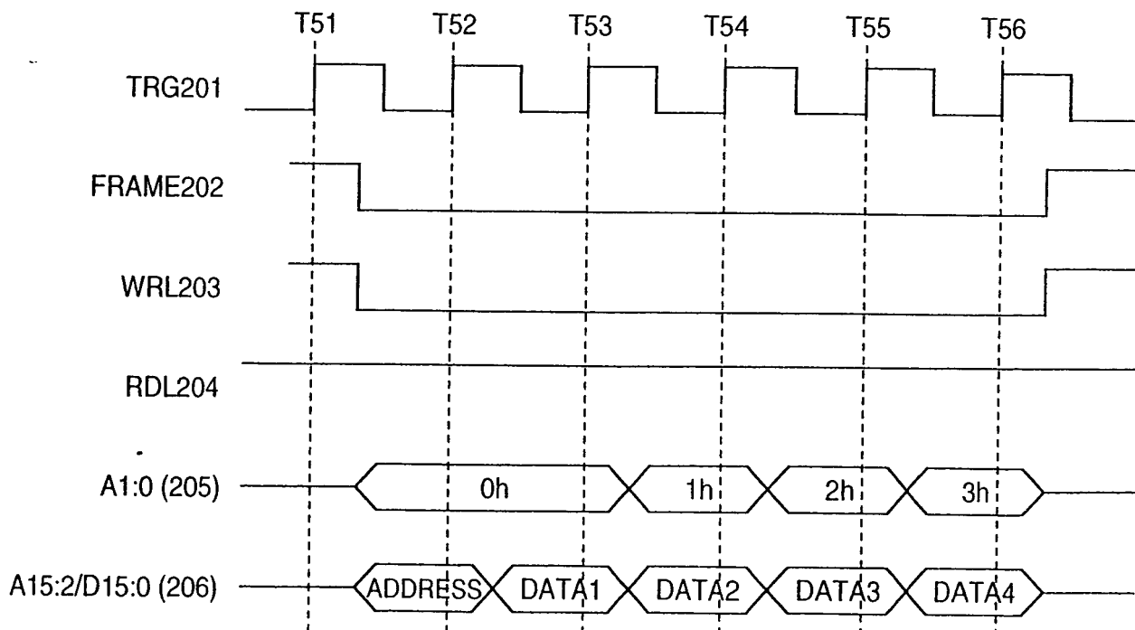
FIG. 22 PRIOR ART
